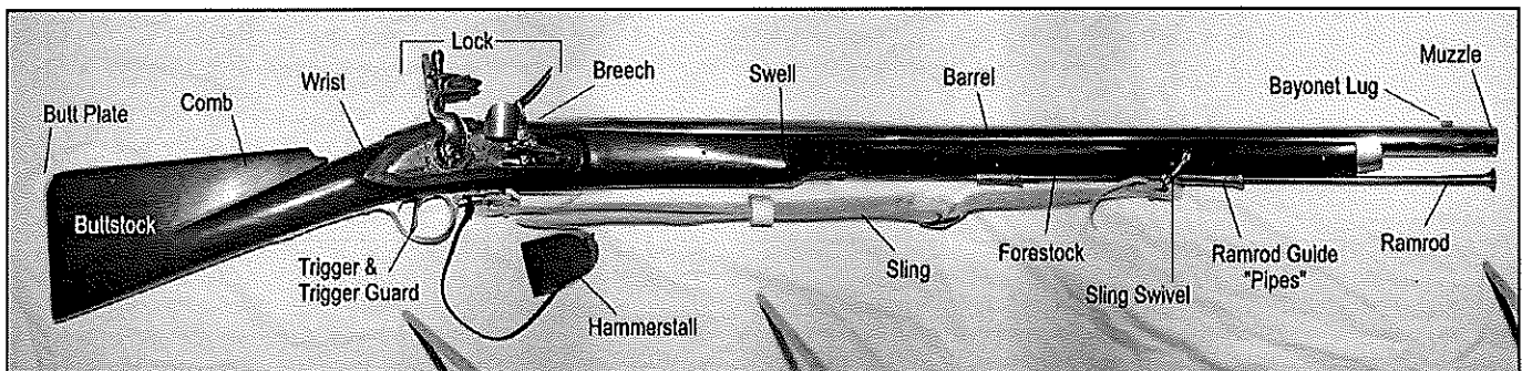
Fig. 6 Parts of a Black Powder Flintlock Musket
