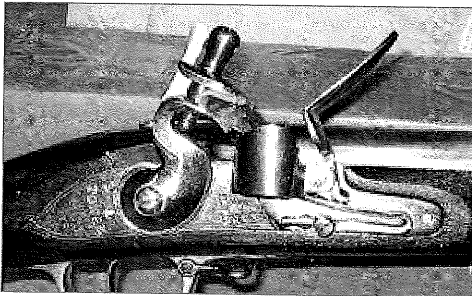
Fig. 1 Flash guard installed on reproduction Brown Bess musket
