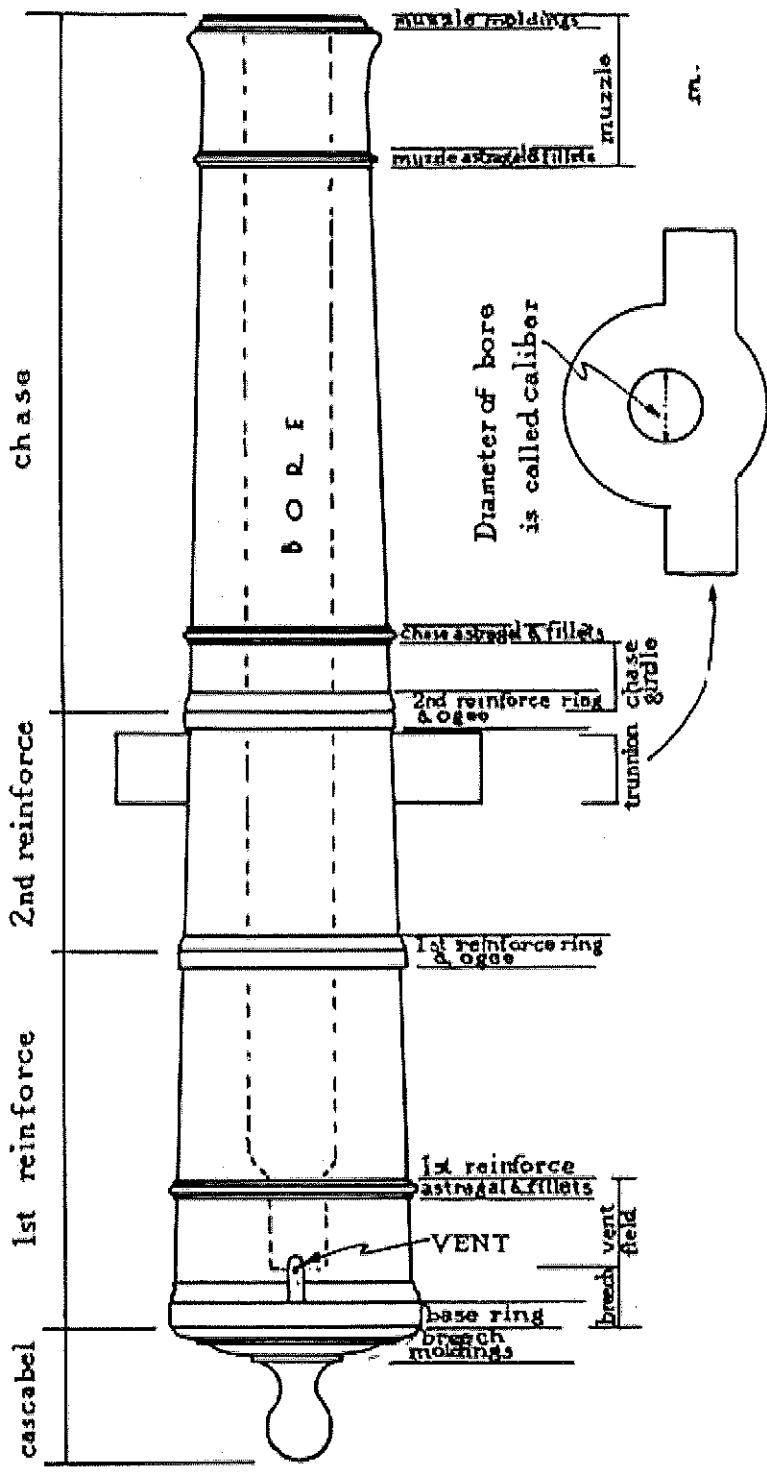
Fig. 7 Basic parts of a cannon tube
