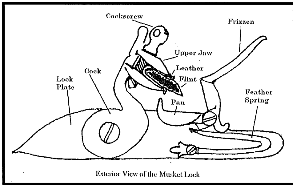
Fig. 7 Parts of a Musket Lock
