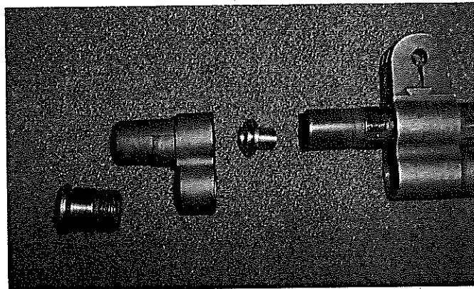
Fig. 3 Threaded “Hollywood” type blank firing adapter for M1 Garand
