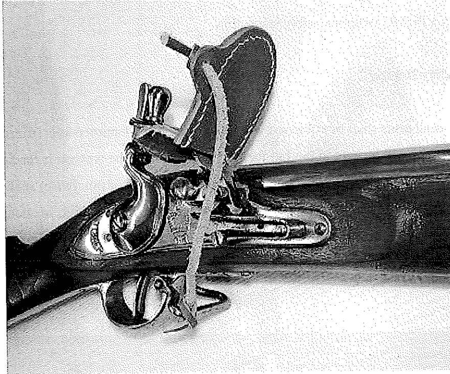
Fig. 2 Frizzen cover or hammerstall
